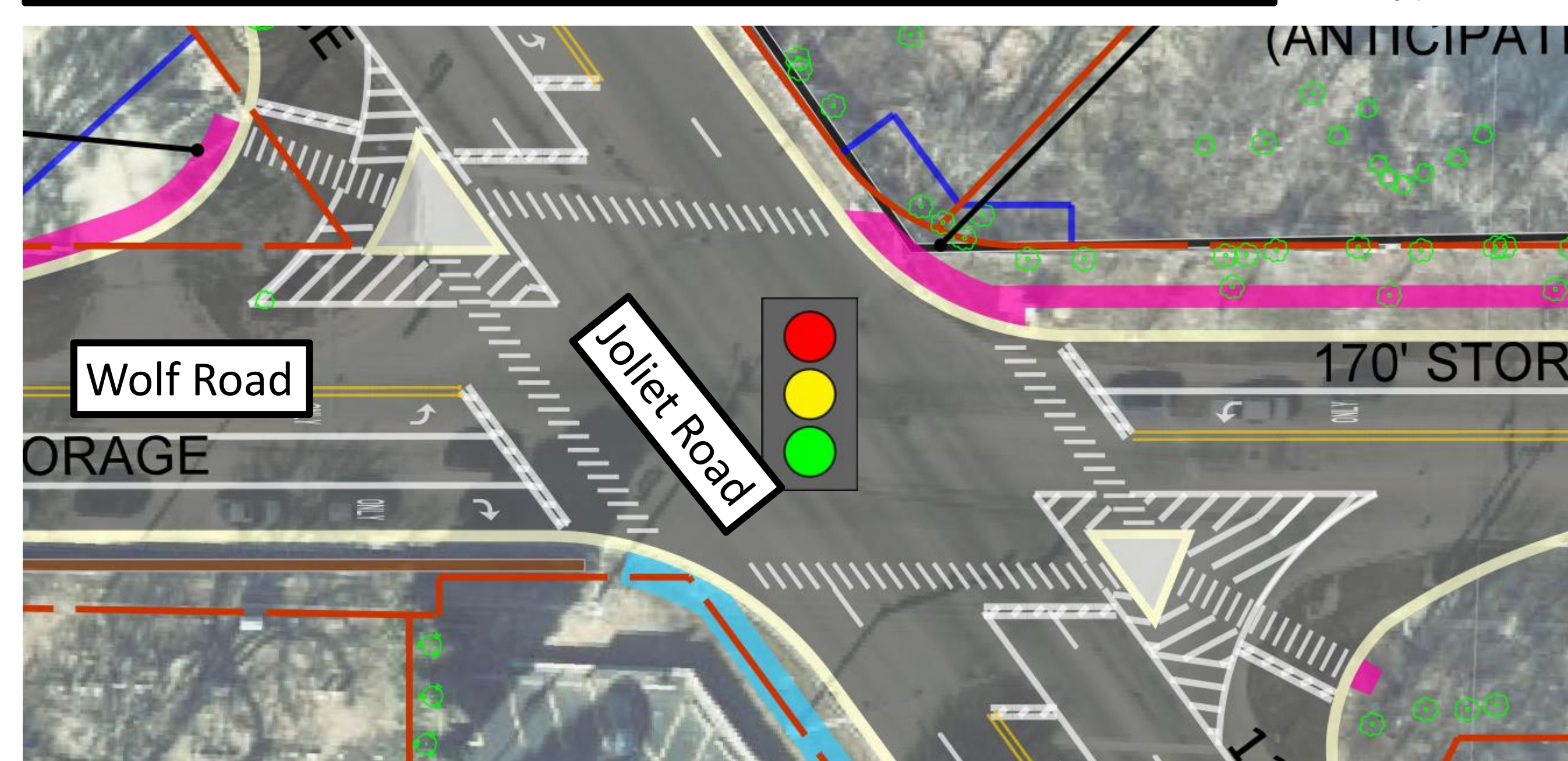
Wolf Road at Joliet Road Signalized Intersection with Pedestrian Refuge
