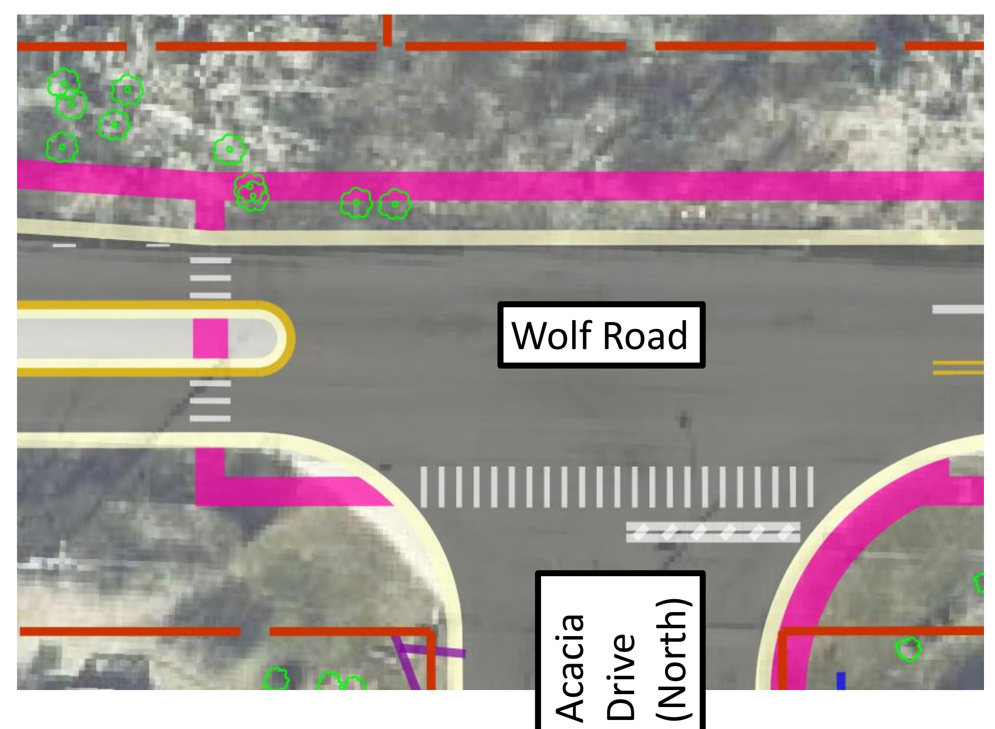
Wolf Road at Acacia Drive (North) Unsignalized Intersection with Pedestrian Refuge
