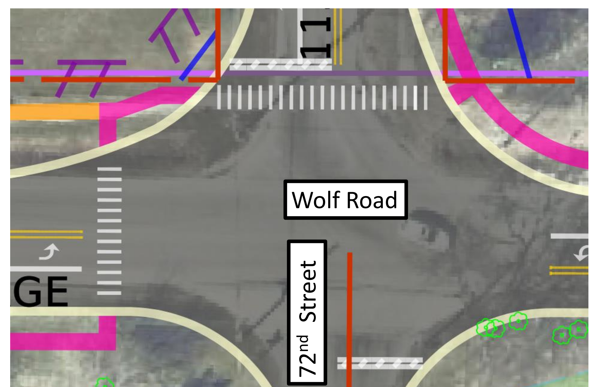
Wolf Road at 72 nd Street Unsignalized Intersection
